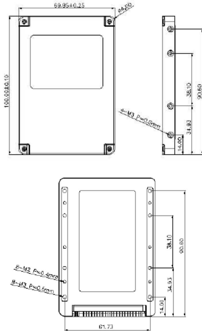
FIGURE 8-1: Physical dimensions
