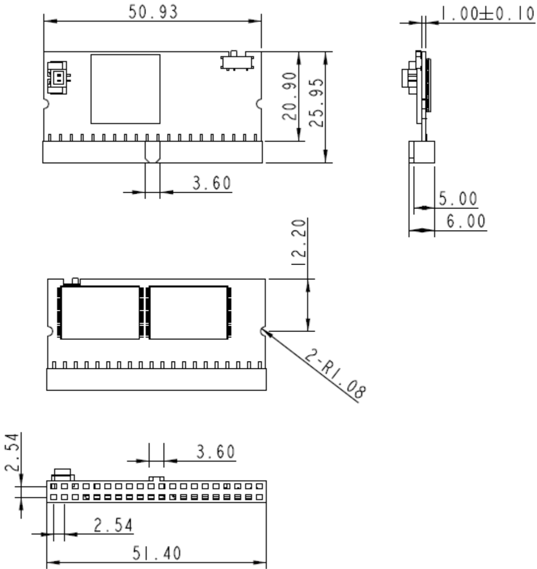
FIGURE 8-1: Physical dimension
