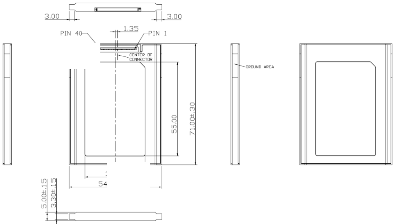
FIGURE 8-1: Physical dimensions
