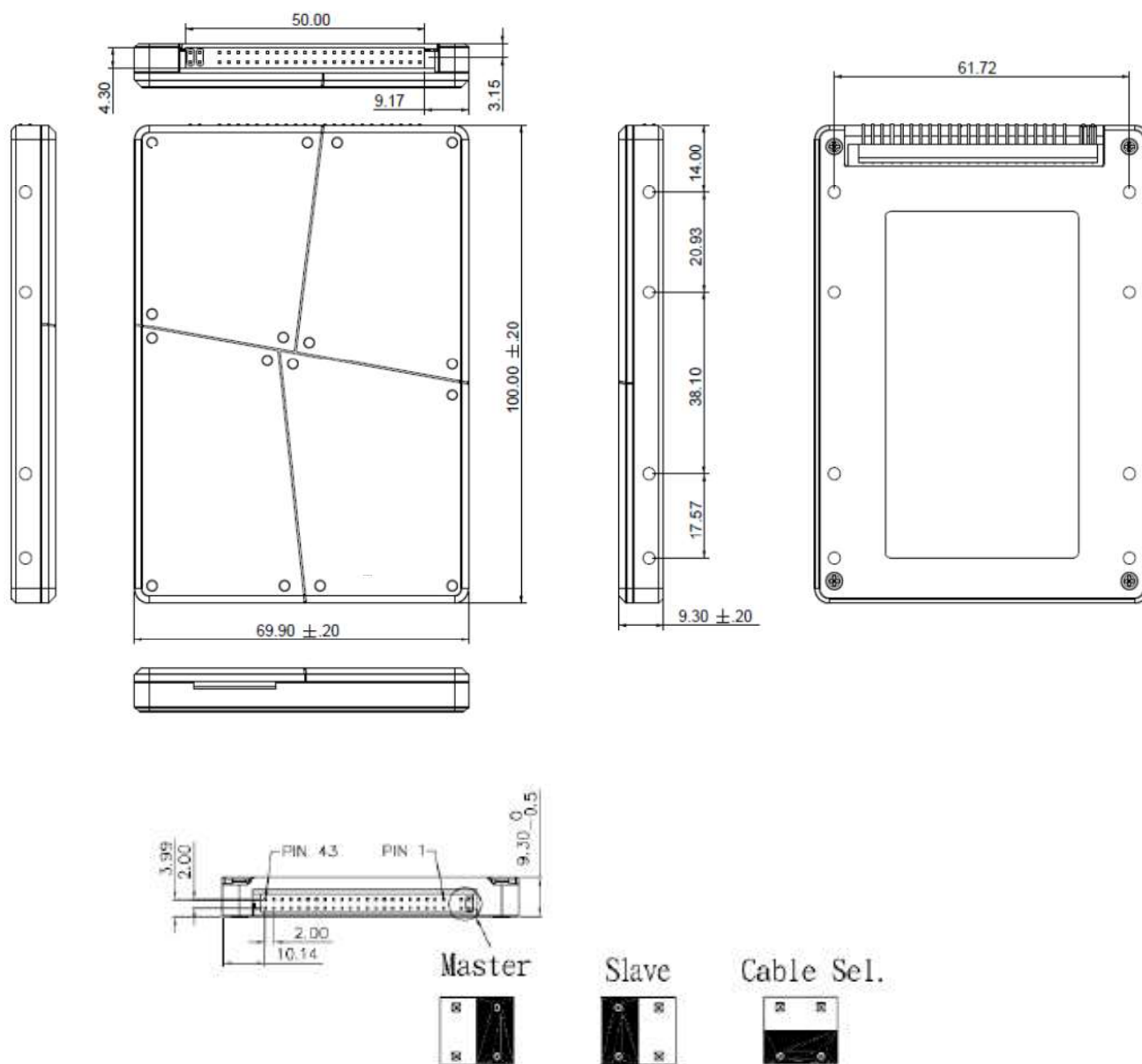
FIGURE 8-1: Physical dimensions
