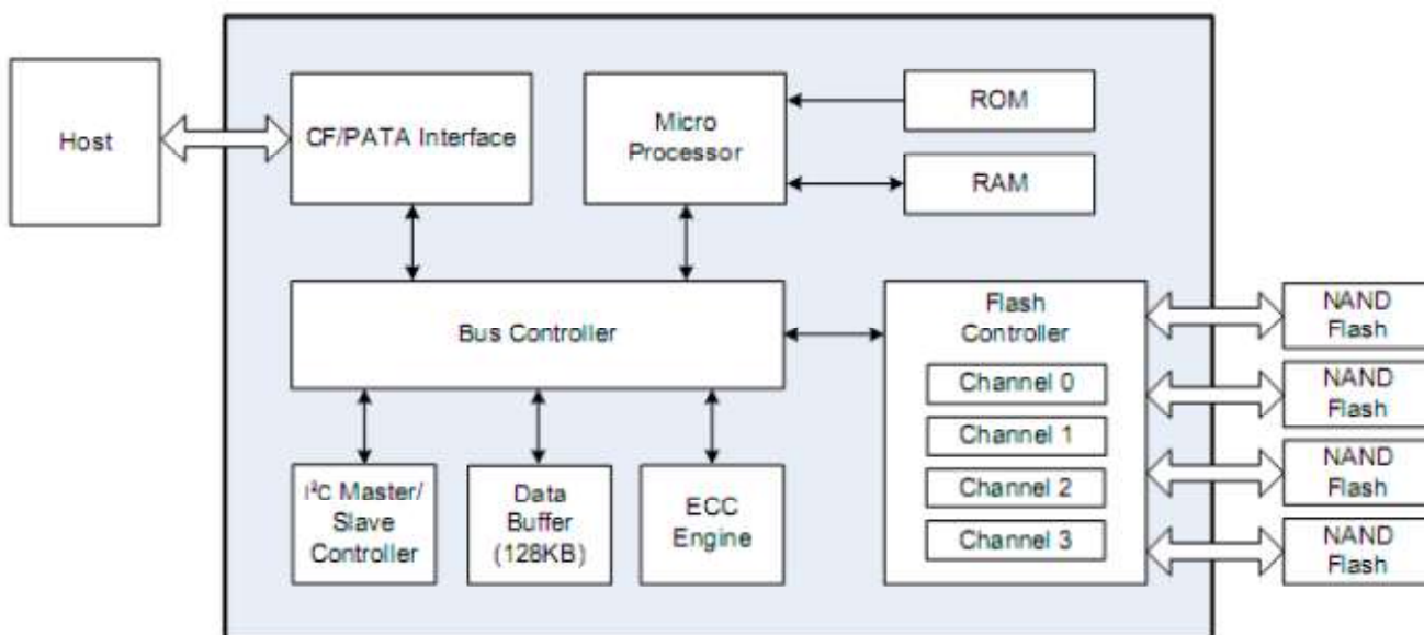
Figure 2-1: Functional block diagram
