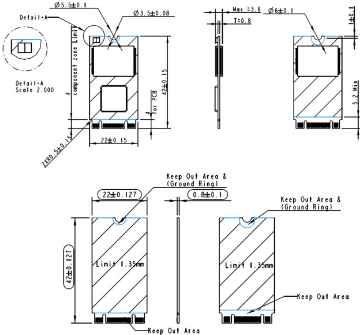
Figure 6-1 M.2 A1 2242 physical dimensions
