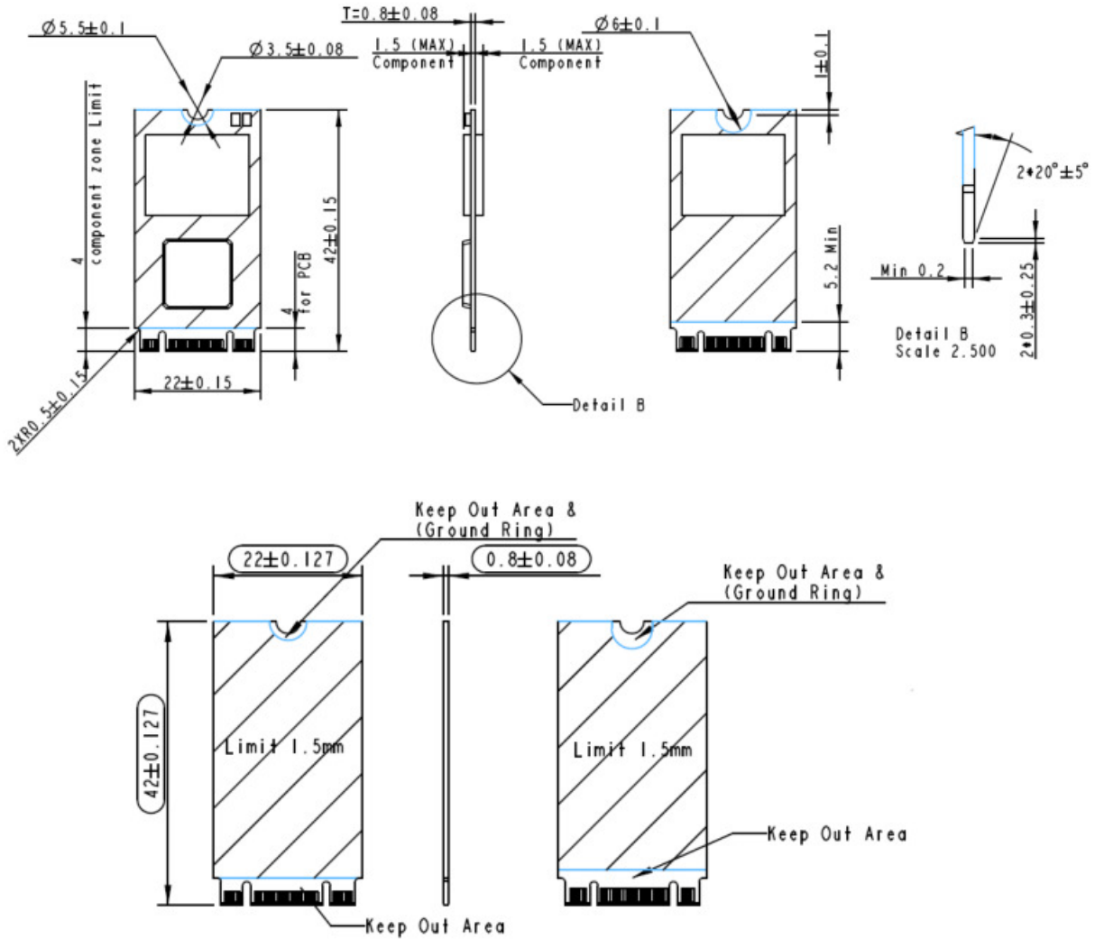
Figure 6-1 M.2 A1 2280 physical dimensions
